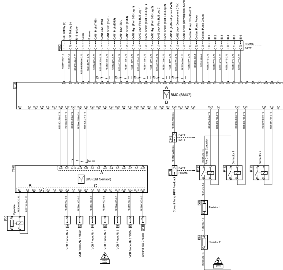
Schematic p/n 2955021: Circuit diagram RES for chassis frame / MegaStructure
